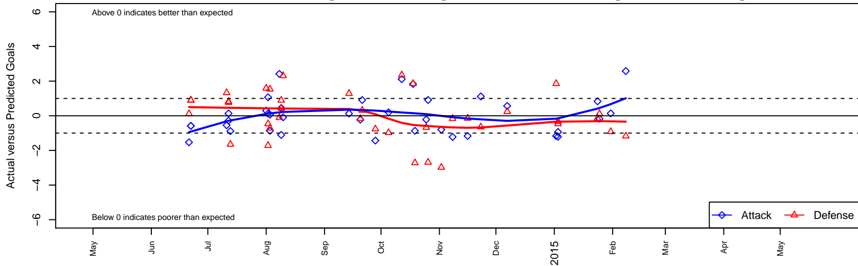
WA Rush B97 Dots are actual minus expected GF (blue circles) and GA (red triangles). Blue line is smoothed change in attack strength. Red is smoothed change in defense strength.
